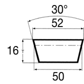
SECTION 52X16 W50
