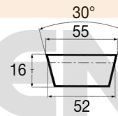
SECTION 55X16
