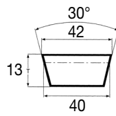
SECTION 42X13 W40
