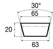
SECTION 65X20 W63
