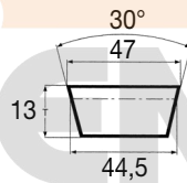
SECTION 47X13
