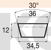
SECTION 36X12
