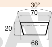
SECTION 70X20
